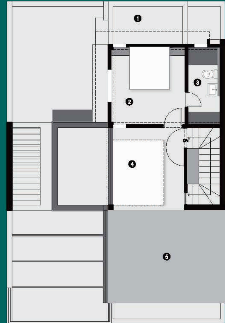
Second Floor (Sloping Roof)
