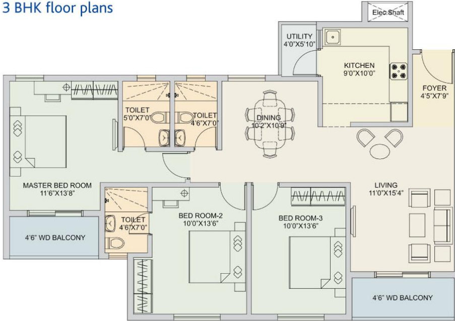
3 BHK LARGE (Size - 1380 Sq. Ft.)
