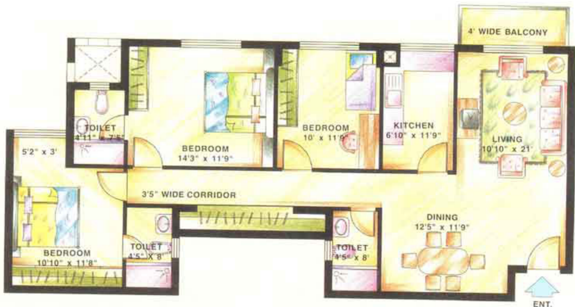
UNIT 2: ACCOMMODATION: Living-Dining with Balcony, 3 Bedrooms, Kitchen and 3 Toilets. AREA: 1396 sq.ft.
