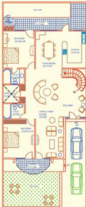
Ground Floor Plan Ground Floor Area = 1681.0 Sft.
