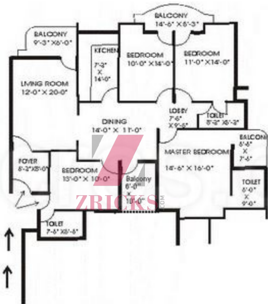
TYPICAL UNIT PLAN
