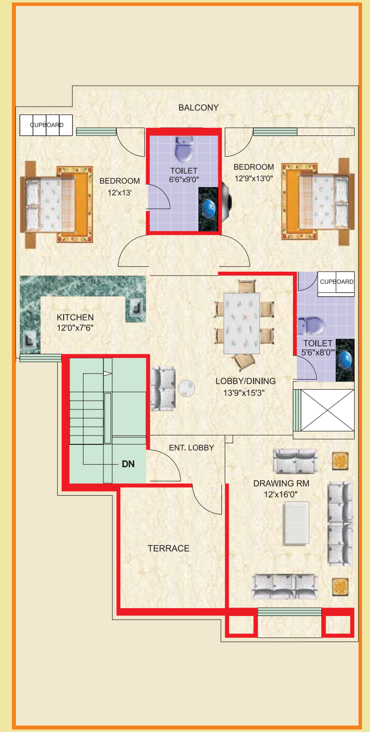
FIRST FLOOR PLAN TOTAL COVERED AREA = 1240 SQ FT
