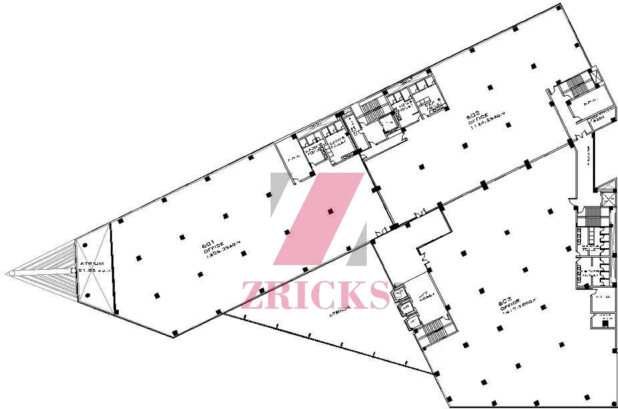
SIXTH FLOOR PLAN
