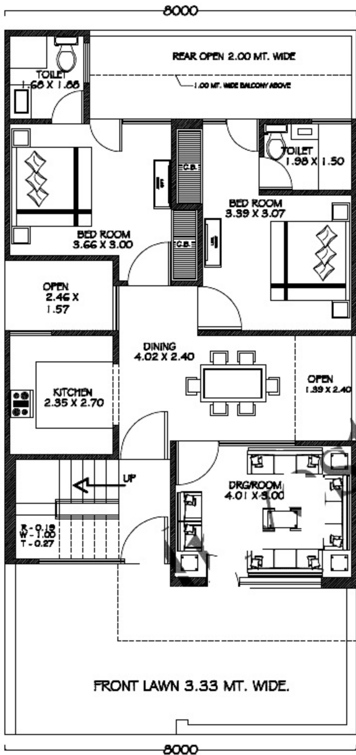
OPTION -01 GROUND FLOOR PLAN PLOT AREA = 128.00 SQ MT
