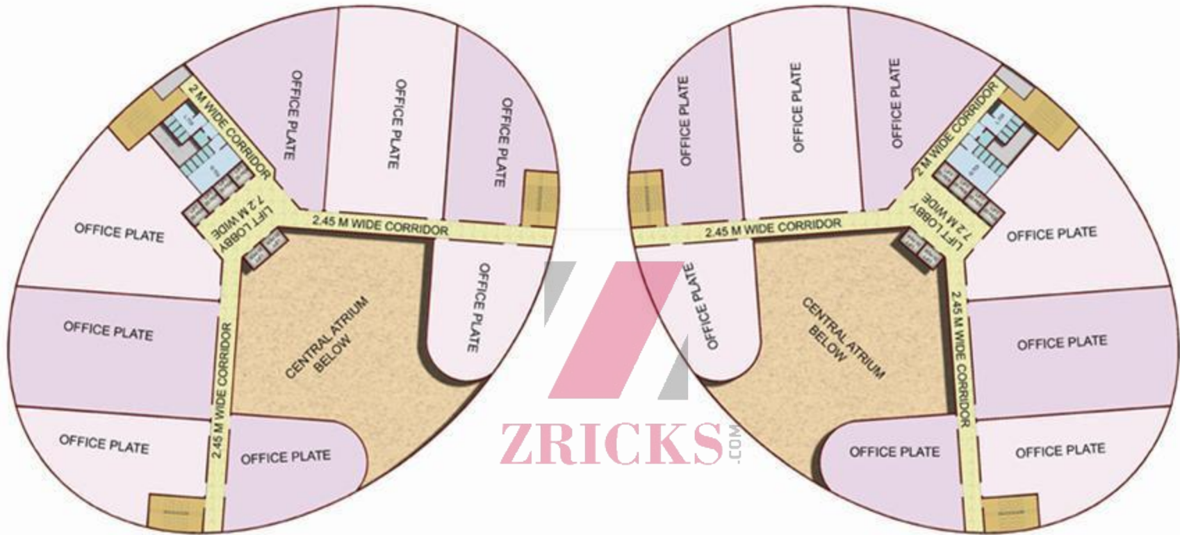
TYPICAL FLOOR PLAN (IT- TOWER)
