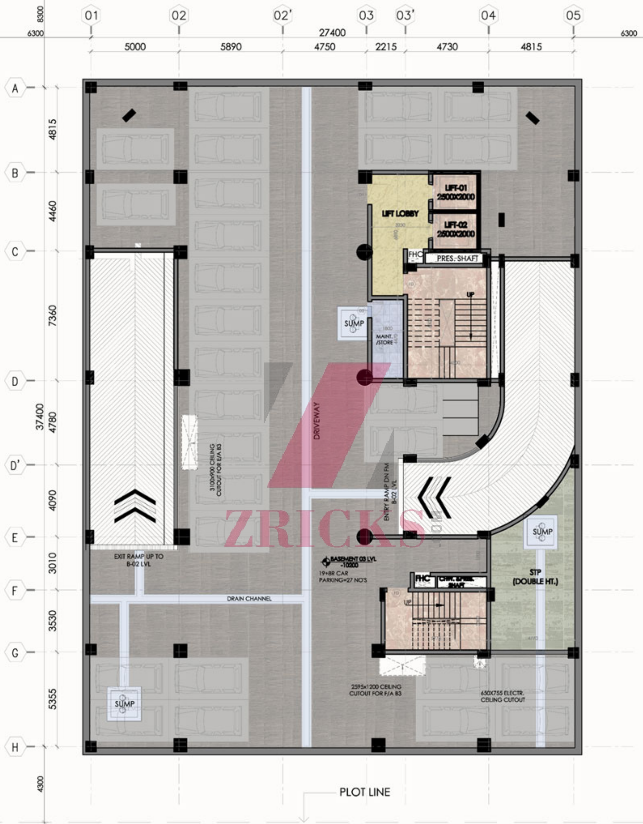
BASEMENT 3 PLAN
