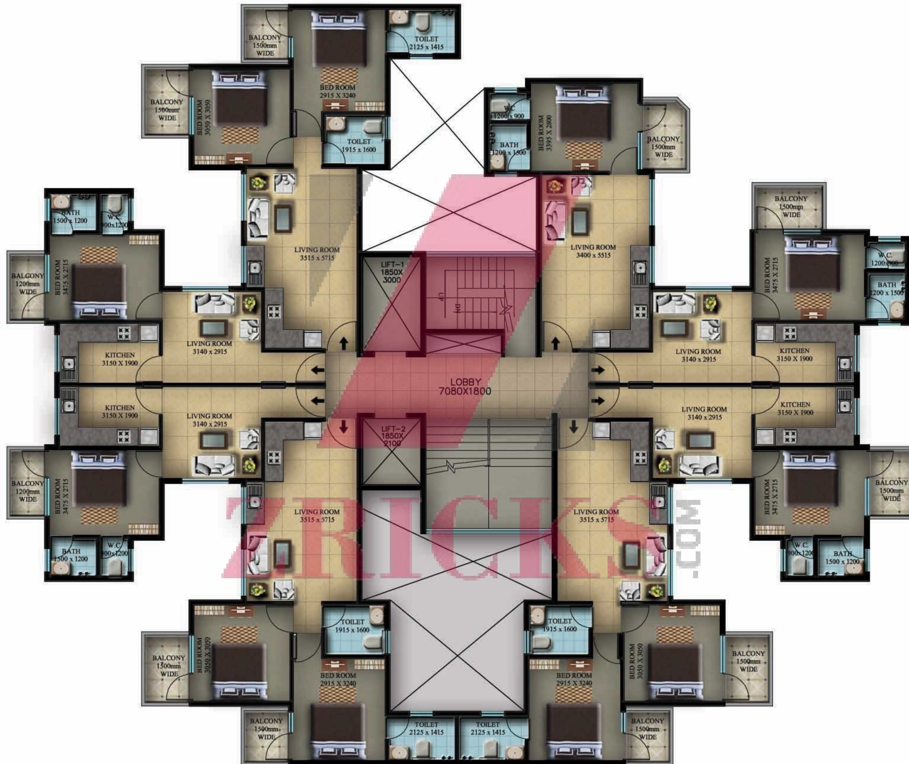
TOWER 7 TYPICAL FLOOR (1 ST - 13 TH )
