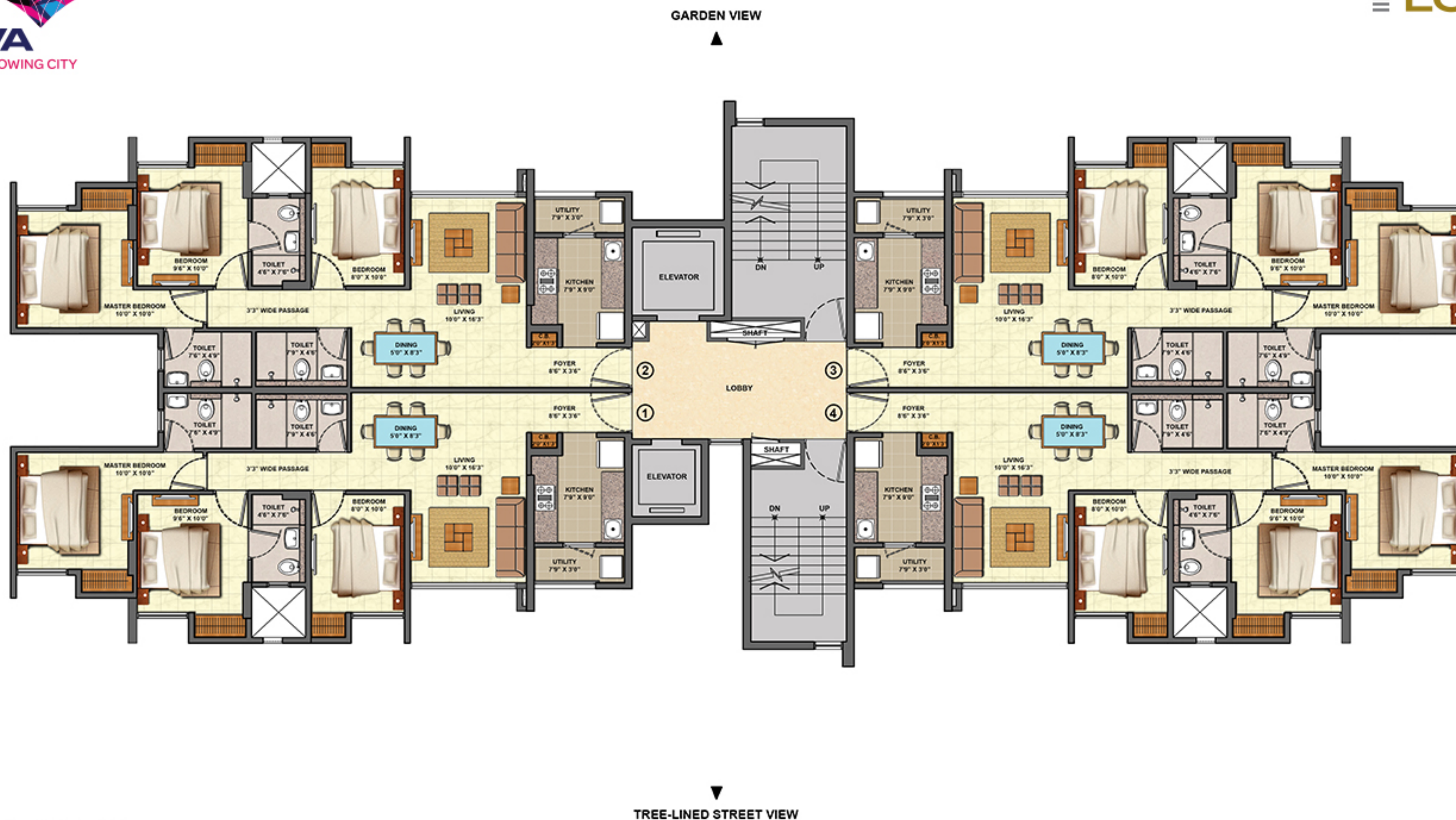
3 BHK ULTIMA TYPICAL UNIT PLAN
