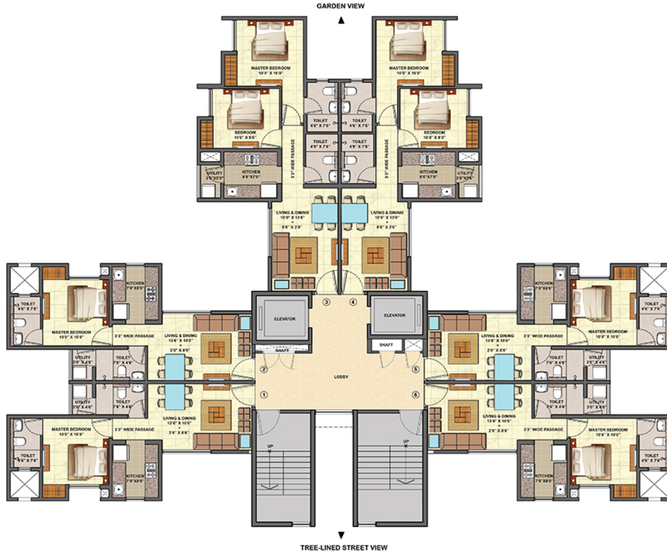
1 BHK & 2 BHK ULTIMA TYPICAL UNIT PLAN (1 TO 7, 9 TO 12 & 15 TO 18)
