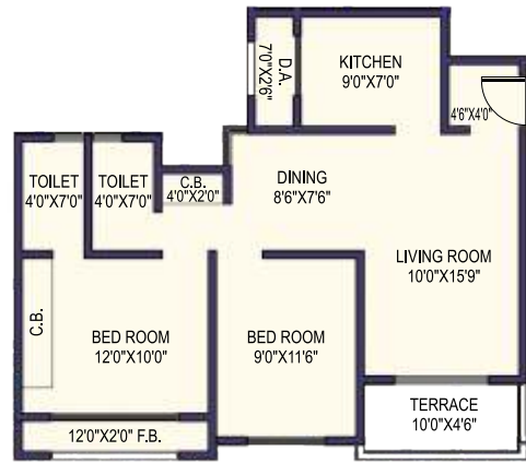
2 BHK Flat Plan
