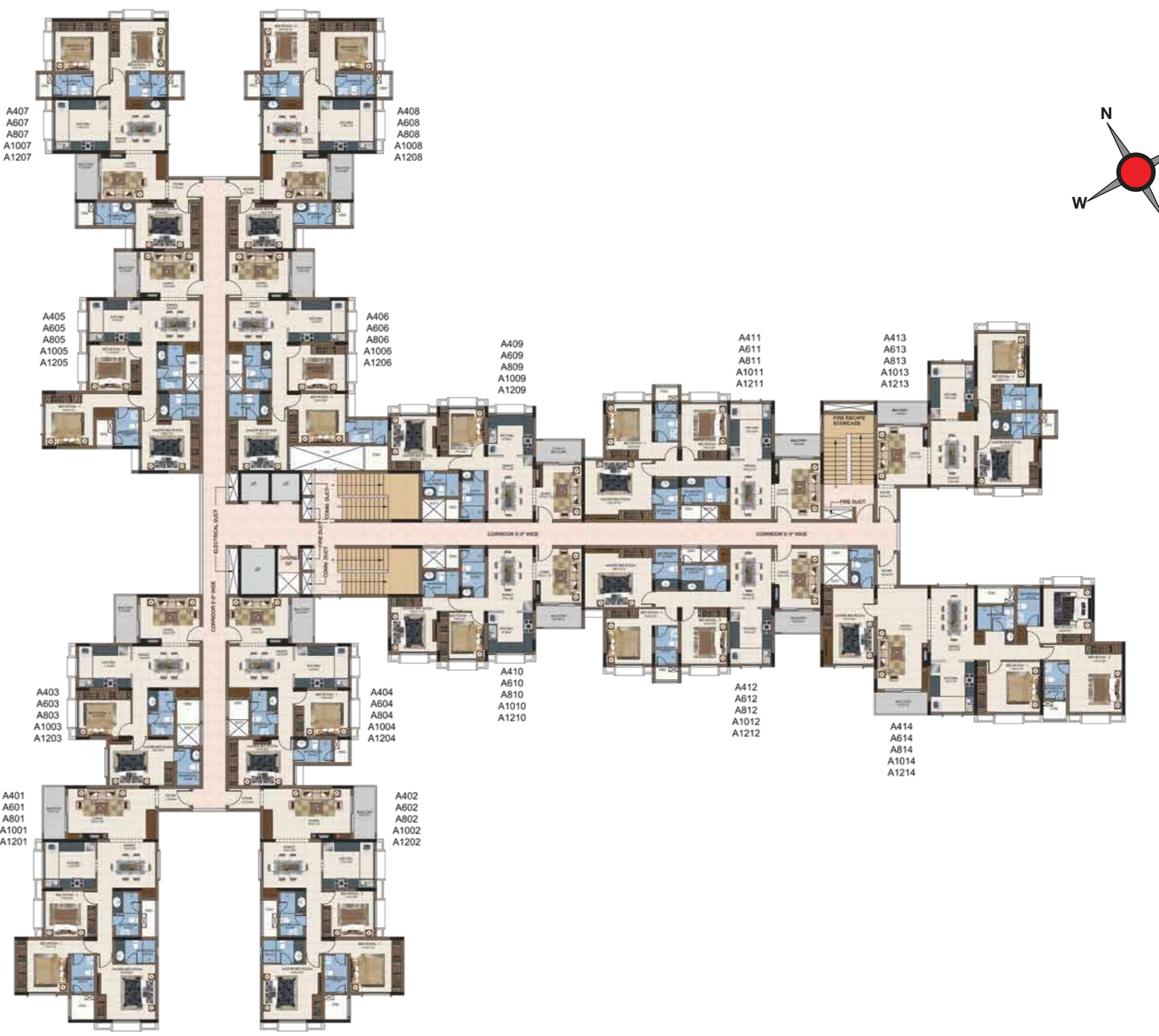
Block - A: 4 th , 6 th , 8 th , 10 th and 12 th floor plan
