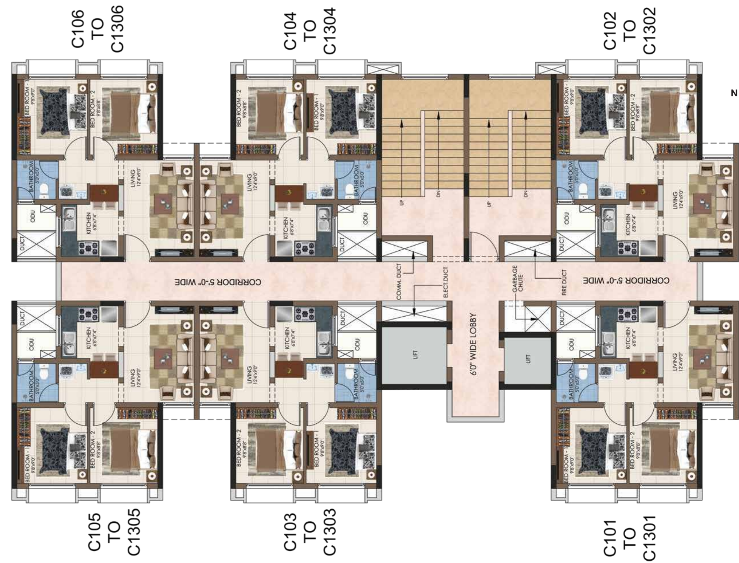
Block - C: 2 nd to 13 th floor plan
